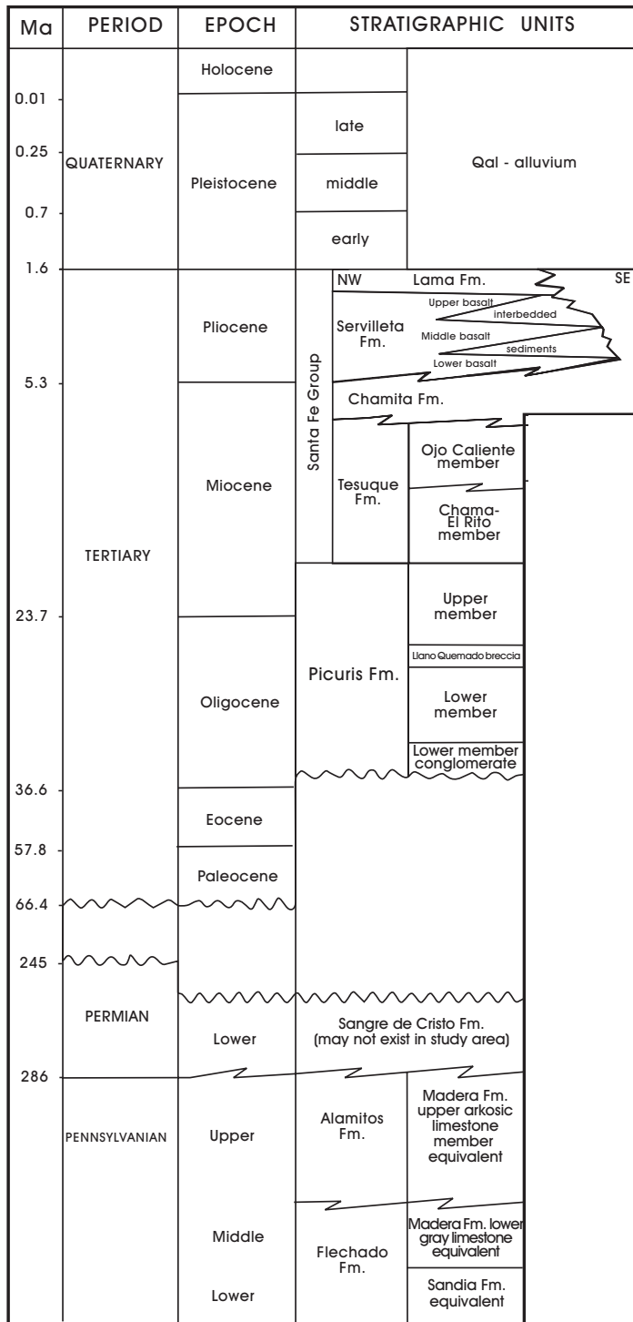
FIGURE 2. Taos Valley Stratigraphic Nomenclature (modified from Bauer et al., 1999)
